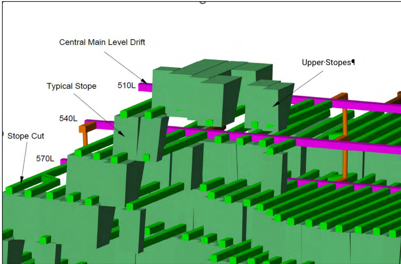
Figure 16-4: Transverse Longhole Stopping in the Santa Cruz Orebody (Looking Southwest)
