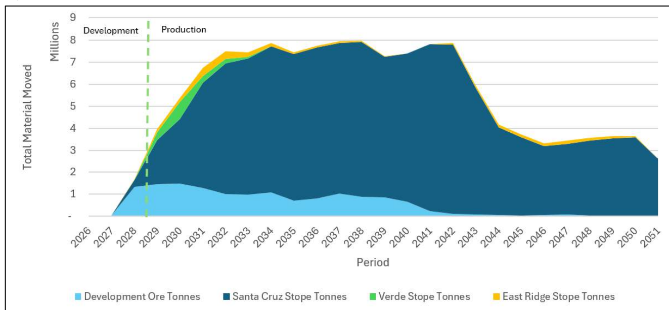
Figure 16-8: Santa Cruz Tonnes of Mined Material
